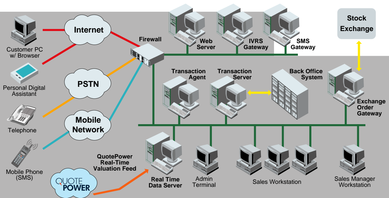
QuotePower - Trade Network
