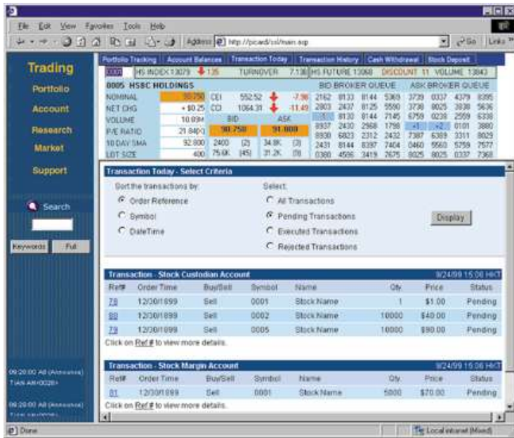
On-line Trading Web Client Showing Trade Status
